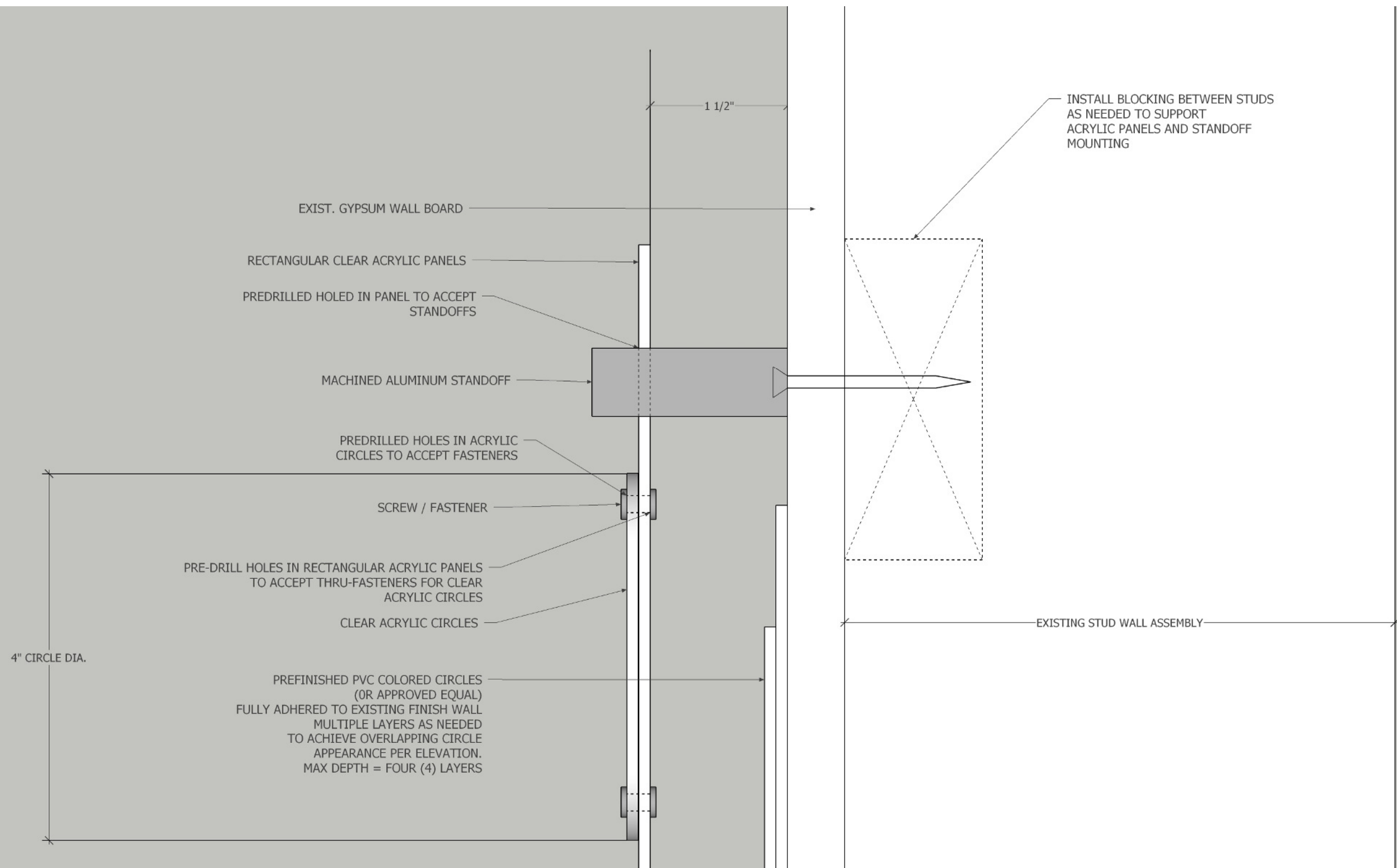
DETAIL (NOT TO A SCALE)
