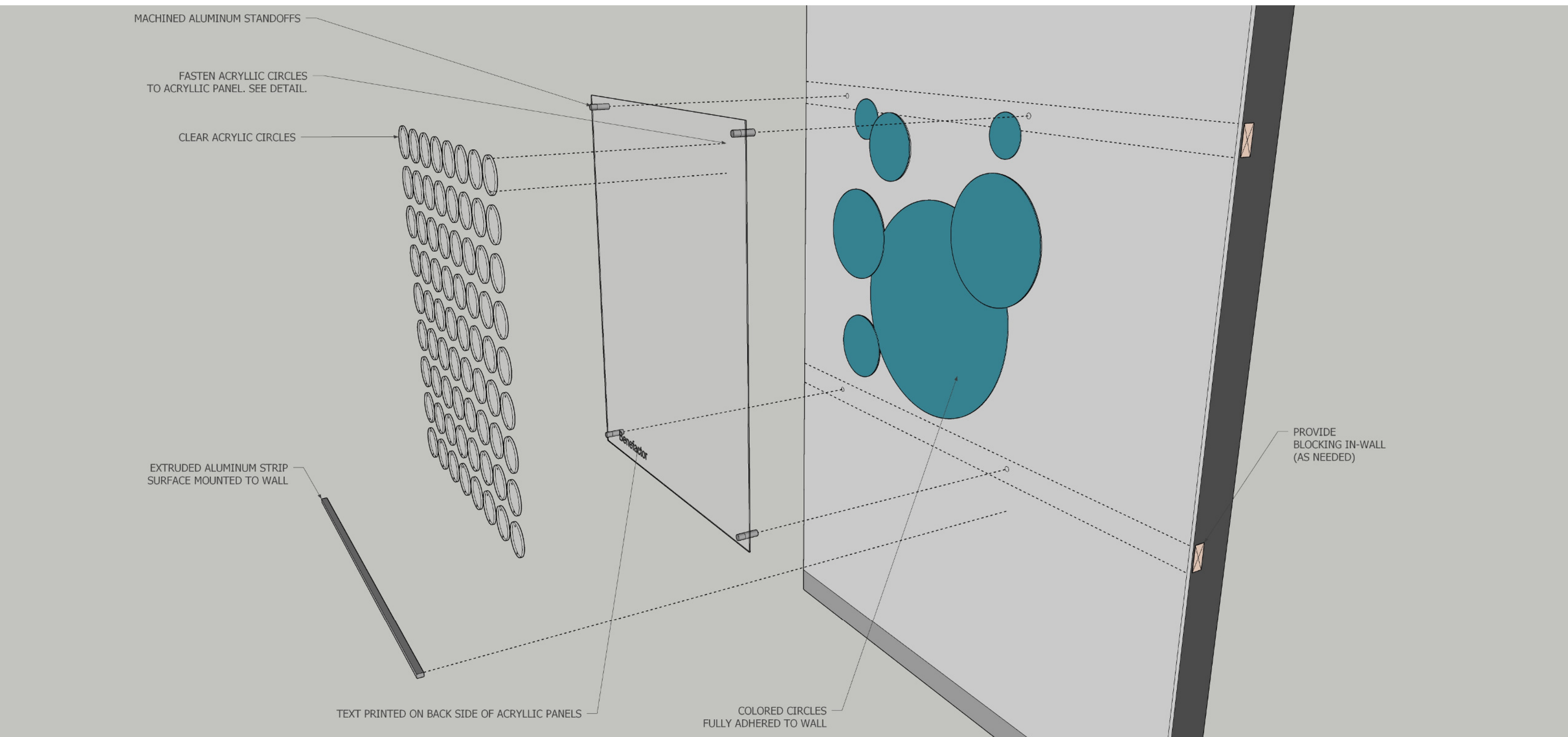
EXPLODED 3D DIAGRAM (NOT TO A SCALE)
