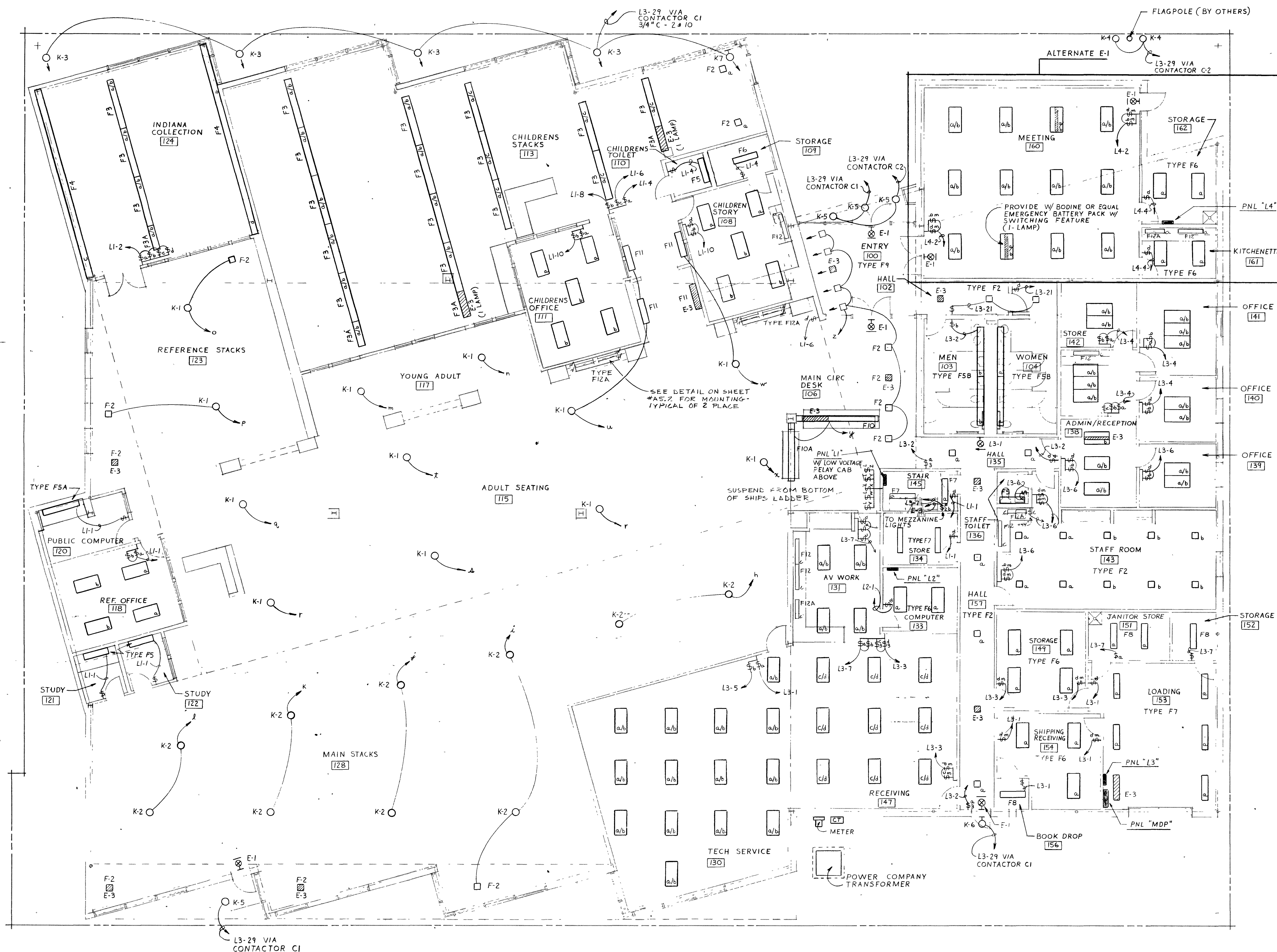
LIGHTING PLAN SCALE: 1/8"=1'-0"
