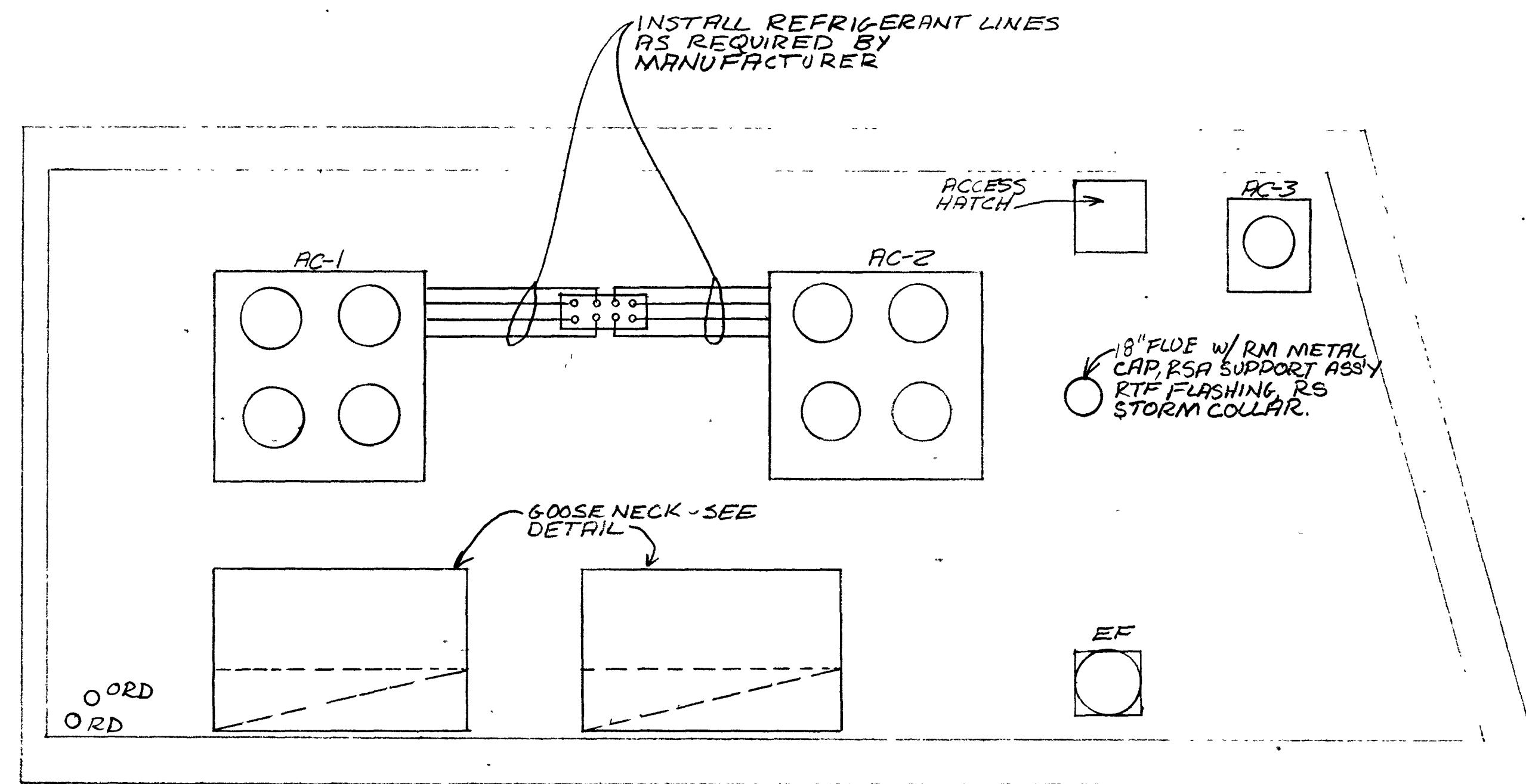
MECHANICAL ROOM ROOF PLAN SCALE 1/4"=1'-0"
