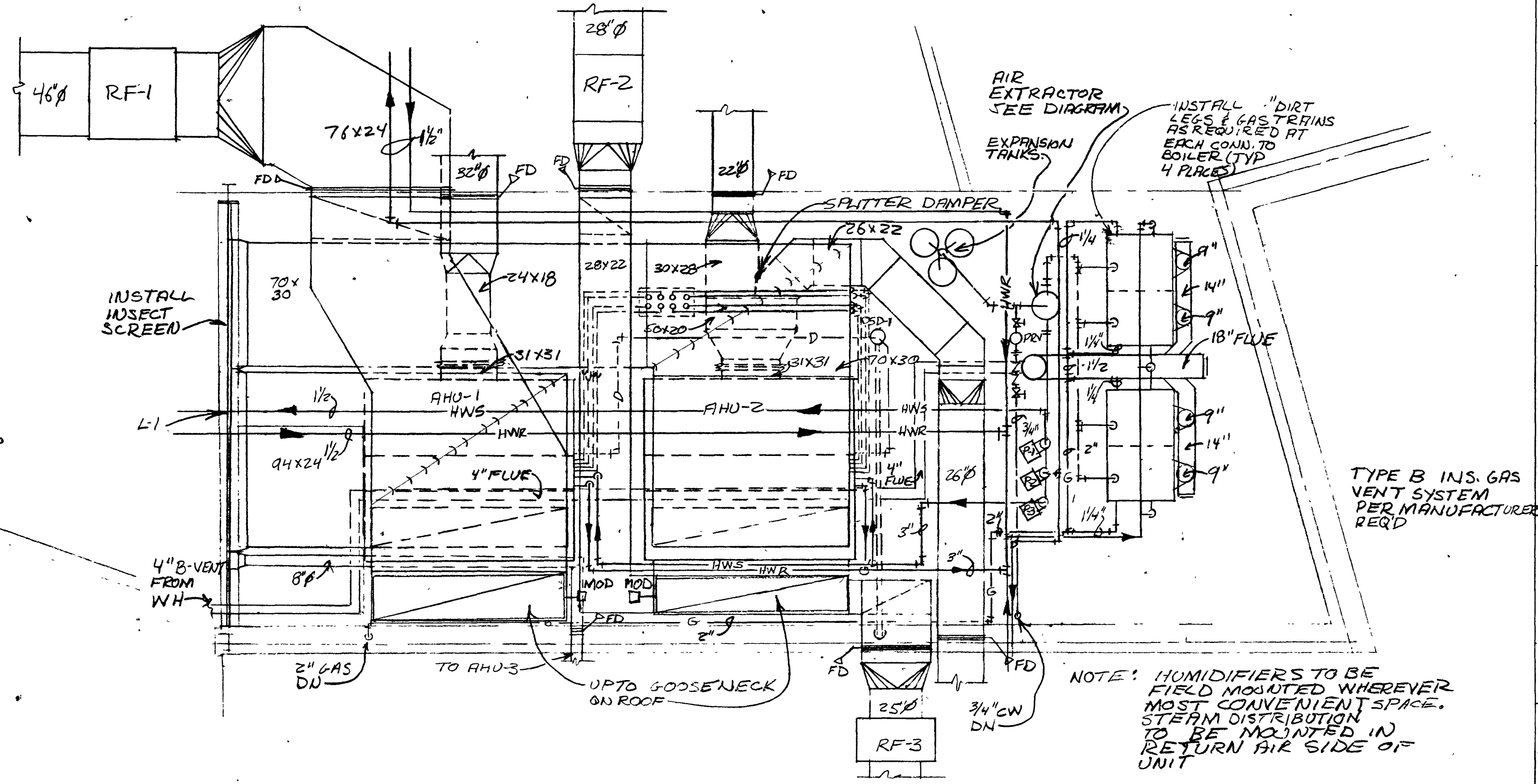
MECHANICAL ROOM PLAN SCALE 1/4"=1'-0"
