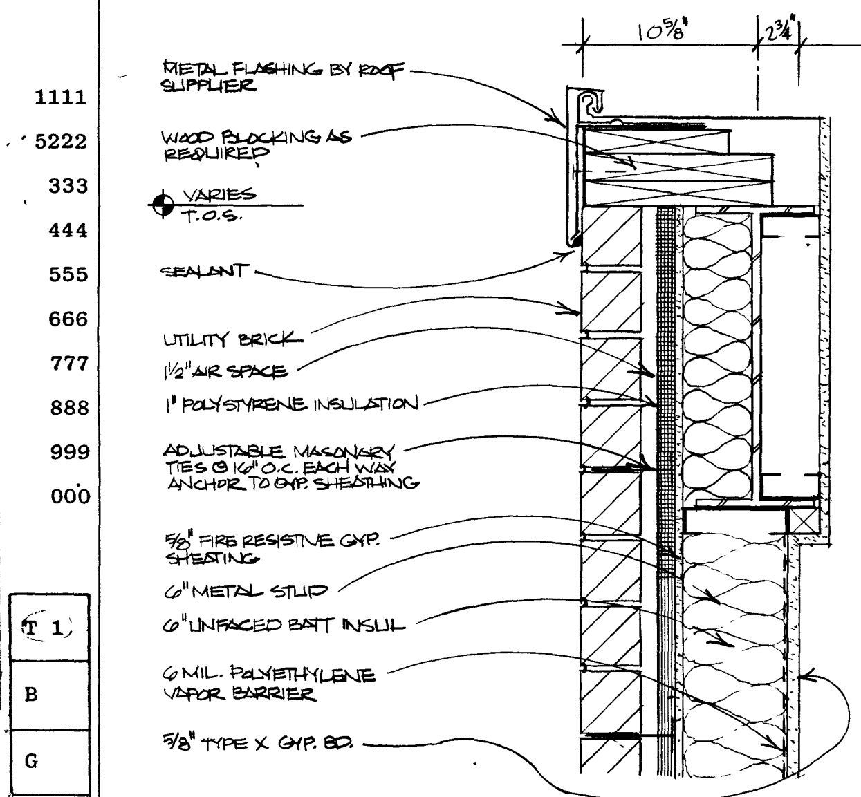
3 DETAIL AT BRICK SIDEWALL A3.3 SCALE: 1/2" = 1'-0"
