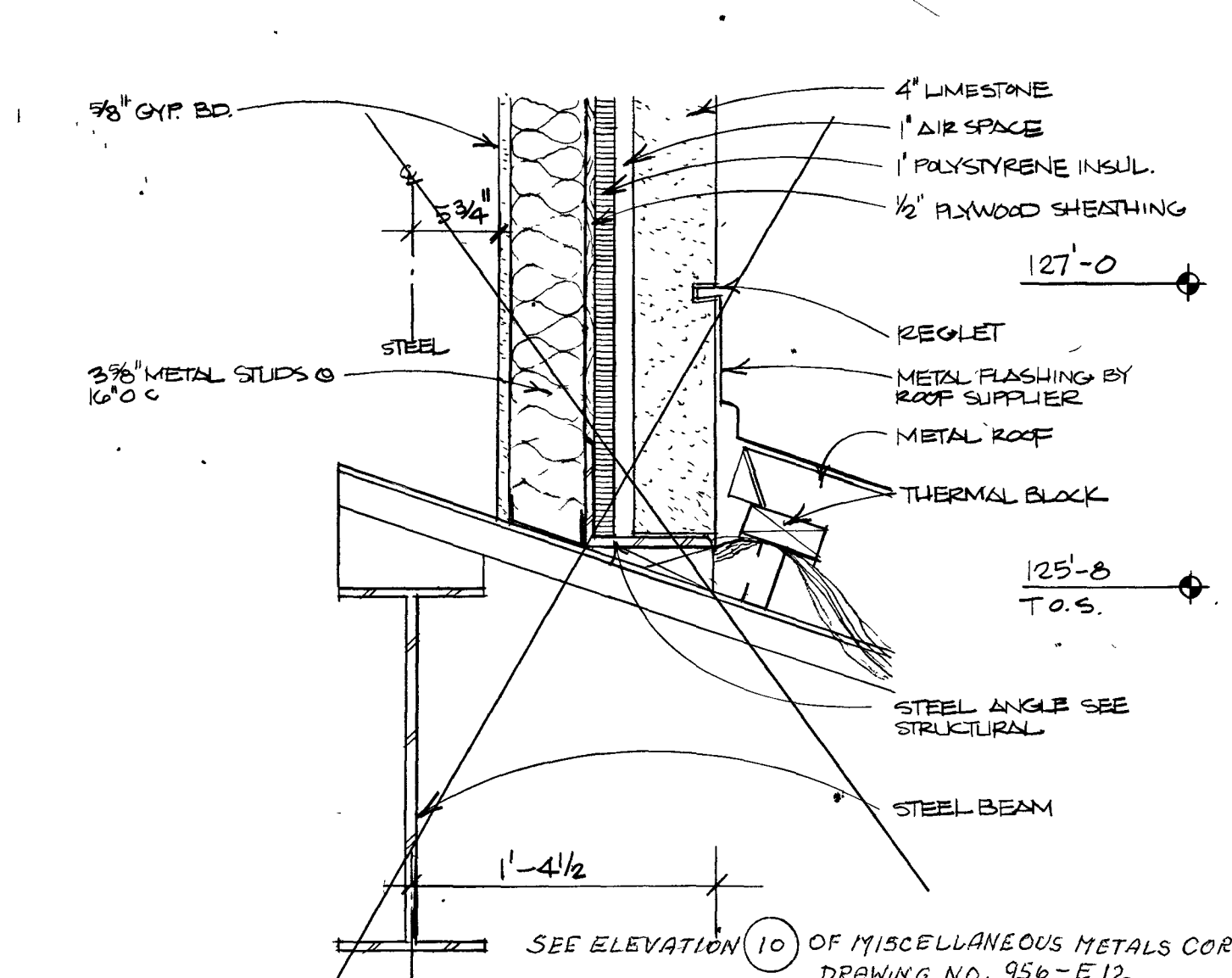
4 DETAIL AT LIMESTONE HEADWALL A3.3 SCALE: 1/2" = 1'-0"
