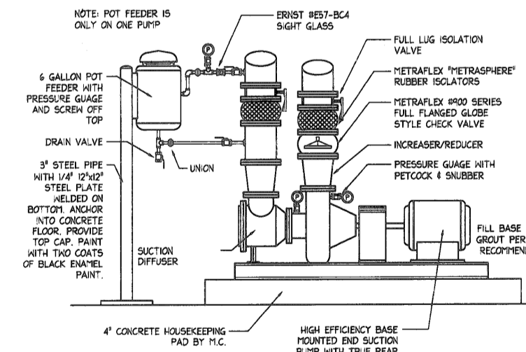
12 TYPICAL BASE MOUNTED PUMP DETAIL SCALE: NTS
