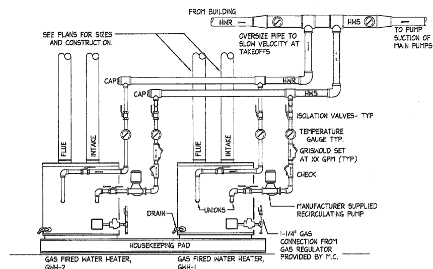
4 WATER BOILER DETAIL SCALE: NTS
