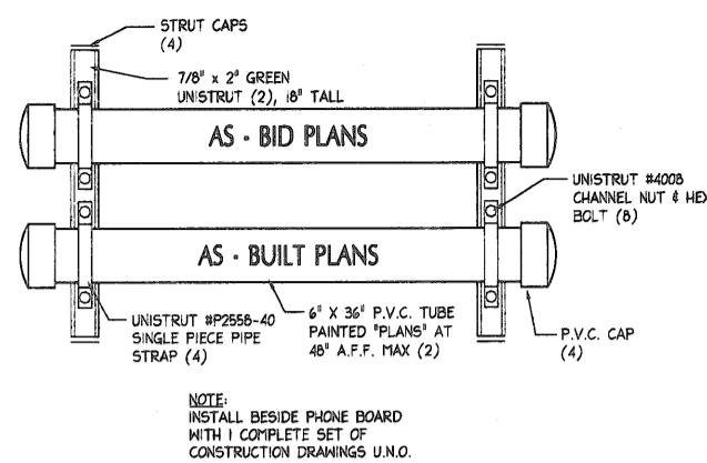
3 PLAN TUBE DETAIL SCALE: NTS
