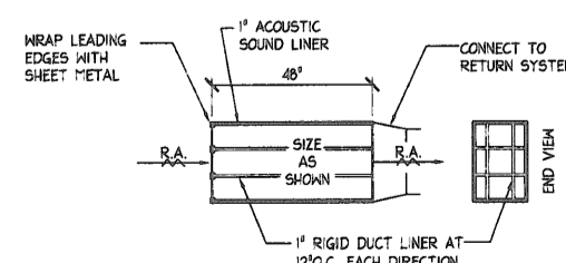
13 SOUND TRAP DETAIL SCALE: NTS
