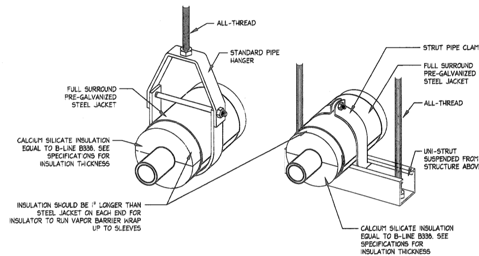
11 TYPICAL PIPE SUPPORT DETAIL SCALE: NTS
