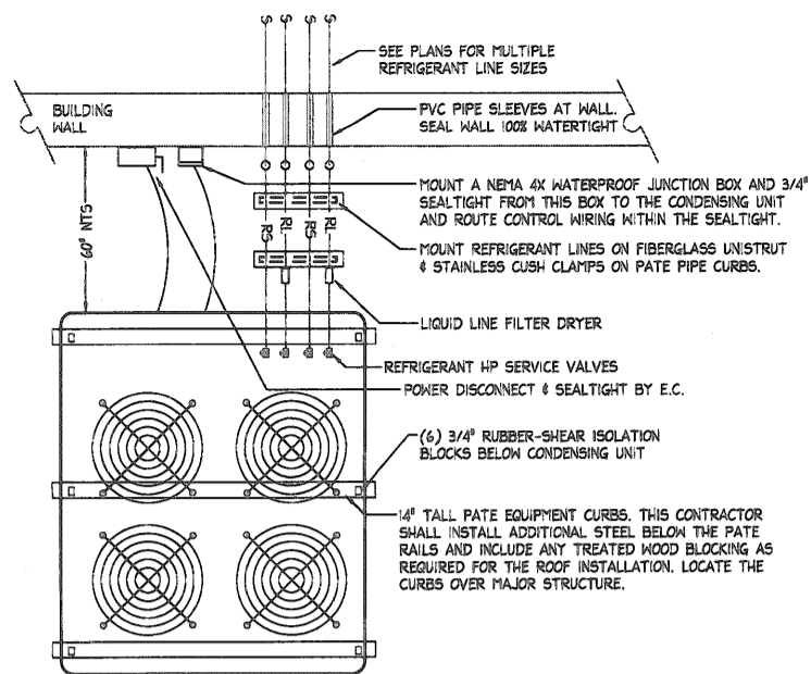
1 TYPICAL CONDENSING UNIT DETAIL SCALE: NTS
