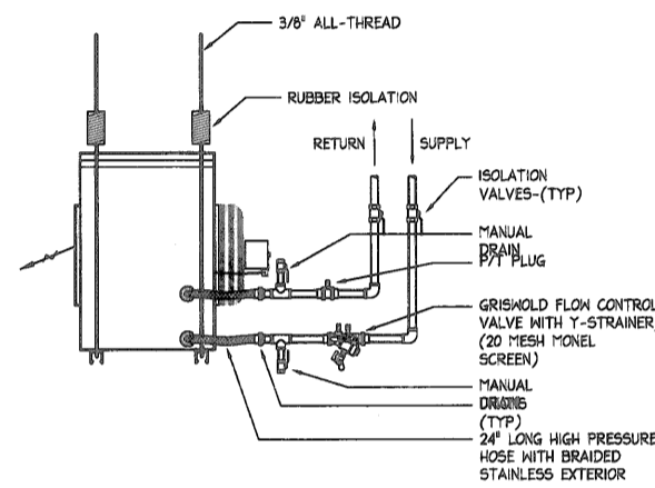
6 TYPICAL UNIT HEATER DETAIL SCALE: NTS
