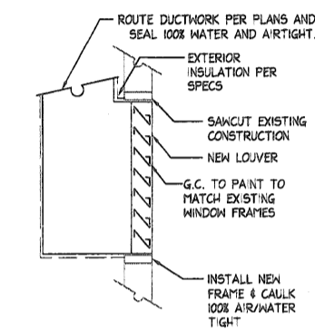
5 TYPICAL "PATCH" RELIEF DETAIL SCALE: NTS
