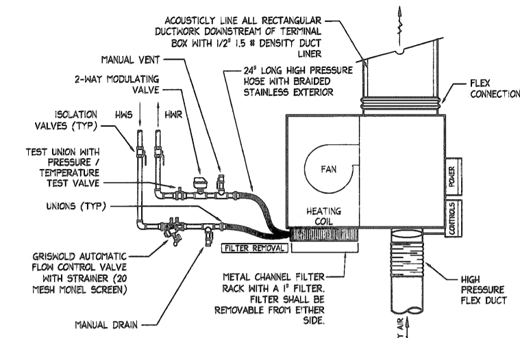
2 TYPICAL FAN POWERED TERMINAL BOX DETAIL SCALE: NTS
