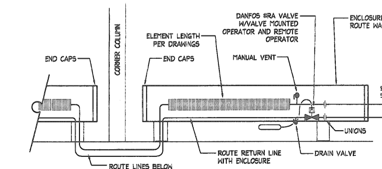
9 TYPICAL PEDestal MOUNTED FIN-TUBE DETAIL SCALE: NTS
