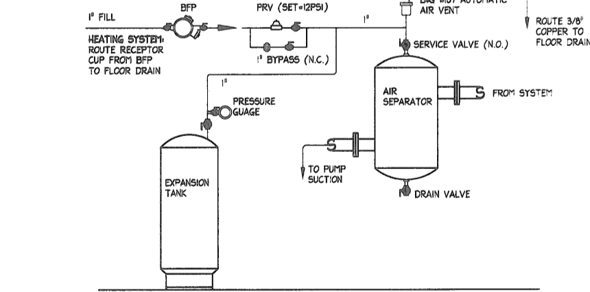
10 TYPICAL AIR SEPARATOR DETAIL SCALE: NTS
