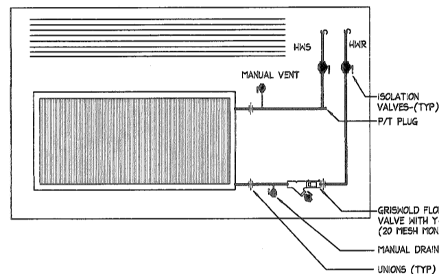
7 TYPICAL CABINET HEATER DETAIL SCALE: NTS
