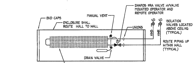
8 TYPICAL WALL MOUNTED FIN-TUBE DETAIL SCALE: NTS
