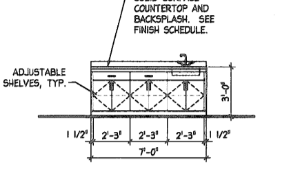
5 CASEWORK ELEVATION SCALE: 1/4" = 1'-0" CAFE 104
