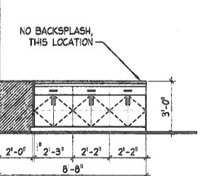
22 CASEWORK ELEVATION SCALE: 1/4" = 1'-0" CHILDREN'S CIRCULATION DESK 147
