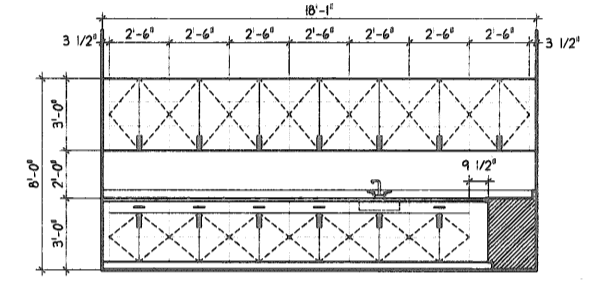
14 CASEWORK ELEVATION SCALE: 1/4" = 1'-0" KITCHEN 129
