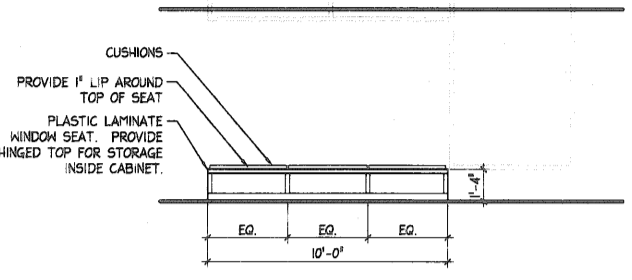
15 CASEWORK ELEVATION SCALE: 1/4" = 1'-0" YOUNG ADULT 127
