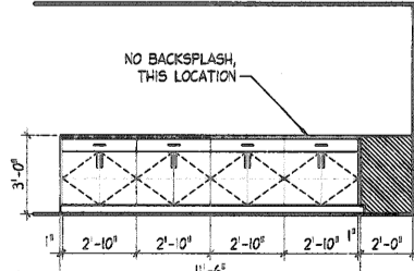
21 CASEWORK ELEVATION SCALE: 1/4" = 1'-0" CHILDREN'S CIRCULATION DESK 147
