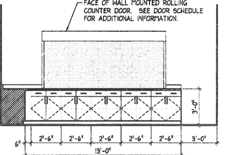
12 CASEWORK ELEVATION SCALE: 1/4" = 1'-0" KITCHEN 129
