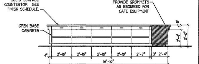
2 CASEWORK ELEVATION SCALE: 1/4" = 1'-0" CAFE 104
