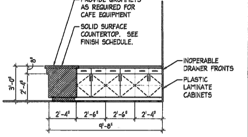
4 CASEWORK ELEVATION SCALE: 1/4" = 1'-0" CAFE 104
