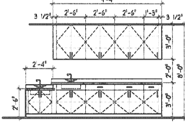
23 CASEWORK ELEVATION SCALE: 1/4" = 1'-0" ART ALCOVE 119
