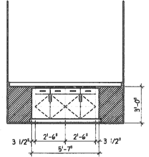
13 CASEWORK ELEVATION SCALE: 1/4" = 1'-0" KITCHEN 129
