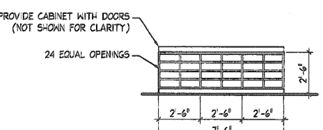
16 CASEWORK ELEVATION SCALE: 1/4" = 1'-0" STORAGE/WORK 140
