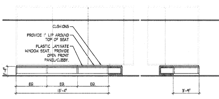
25 CASEWORK ELEVATION SCALE: 1/4" = 1'-0" ART ALCOVE 119
