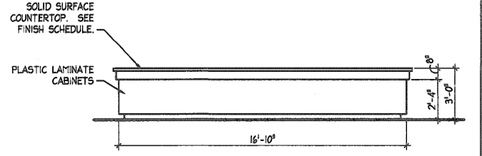
1 CASEWORK ELEVATION SCALE: 1/4" = 1'-0" CAFE 104
