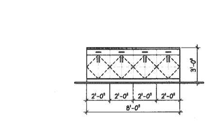
10 CASEWORK ELEVATION SCALE: 1/4" = 1'-0" CIRCULATION DESK 128
