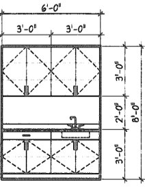
11 CASEWORK ELEVATION SCALE: 1/4" = 1'-0" PROGRAMMING 127
