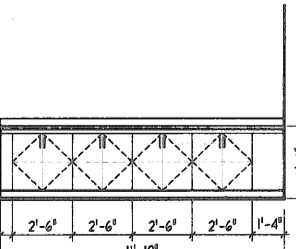
6 CASEWORK ELEVATION SCALE: 1/4" = 1'-0" KITCHENETTE 105
