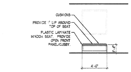
24 CASEWORK ELEVATION SCALE: 1/4" = 1'-0" COLLECTIONS 140
