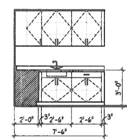
18 CASEWORK ELEVATION SCALE: 1/4" = 1'-0" STORAGE/WORK 140
