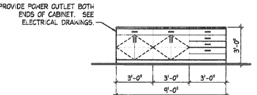
17 CASEWORK ELEVATION SCALE: 1/4" = 1'-0" STORAGE/WORK 140
