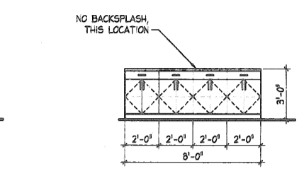
20 CASEWORK ELEVATION SCALE: 1/4" = 1'-0" YOUNG ADULT/REFERENCE DESK 127
