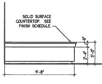
3 CASEWORK ELEVATION SCALE: 1/4" = 1'-0" CAFE 104
